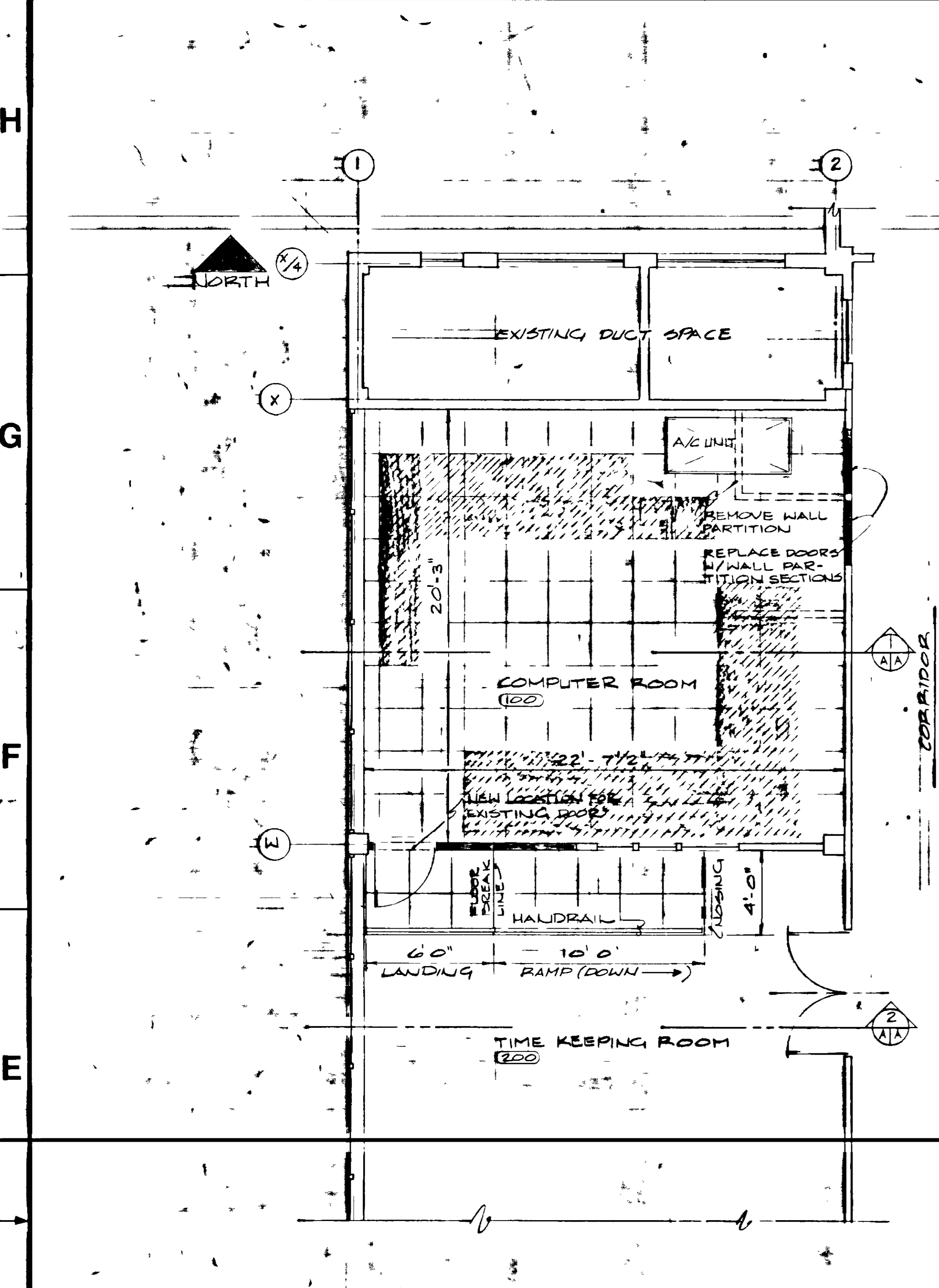
FLOOR PLAN OF COMPUTER ROOM, RAMP LANDING AND RAMP SCALE: 1/4" = 1'-0"
